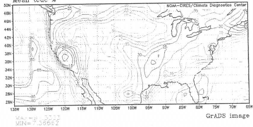
FIG. 5. Mapped 3-day average (12–14 Sep 2001) of (a) anomalies of OLR in W m^{-2} , (b) anomalies of relative humidity at 500 hPa; RH(500) in percent; and (c) mean percentage of total cloud sky coverage, derived using the NCEP–NCAR reanalyses.
