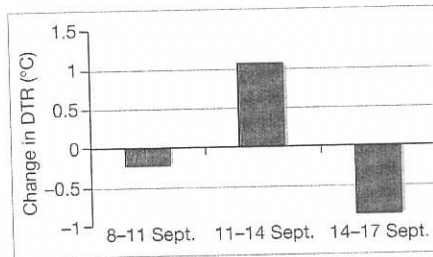
Figure 1 Departure of average diurnal temperature ranges (DTRs) from the normal values derived from 1971-2000 climatology data for the indicated three-day periods in September 2001. These periods included the three days before the terrorist attacks of 11 September; the three days immediately afterwards, when aircraft were grounded and there were therefore no contrails; and the subsequent three days.
